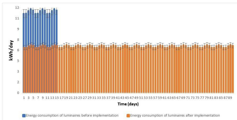
Figure 7. Comparison of daily energy consumption before and after the implementation of green technology in the EFCAUNT module
