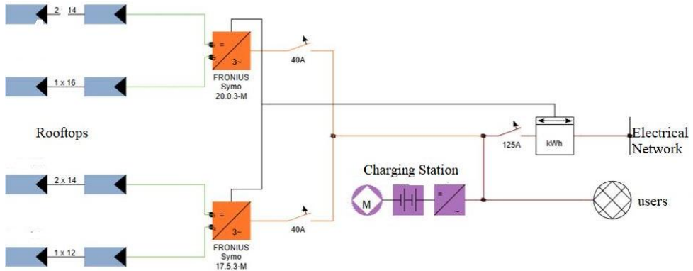
Fig. 1. Basic electrical diagram of the enterprise.
