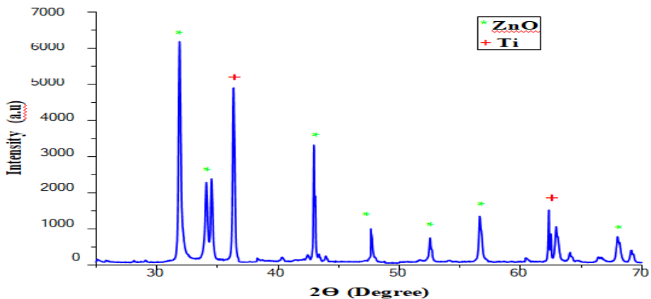
Figure 2. XRD test Results of Ti-doped Zinc nanoparticle
