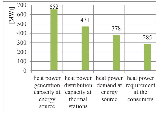
Fig.15. Thermal power production and distribution capacities of the district system of Oradea compared with the heating demand at the level of 2005.
