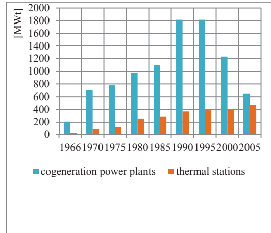
Fig. 13 . Thermal power capacities installed in cogeneration plants of Oradea versus distribution stations
