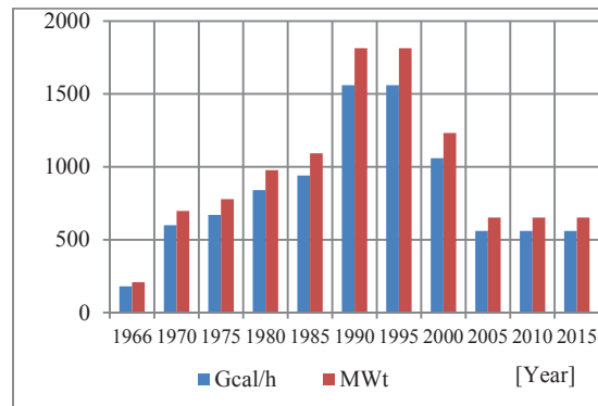
Fig. 10. Hot water preparation capacities installed at the cogeneration power plants Oradea evolving between 1966-2015.
