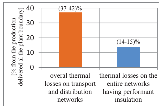
Fig. 18. Thermal losses on the district heating system delivered by the Western Cogeneration Power of Oradea in the year 2014.
