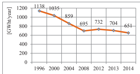
Fig.16. Thermal energy delivered by the Western Cogeneration Plant of Oradea at the consumers inlet in the period 1996-2014.
