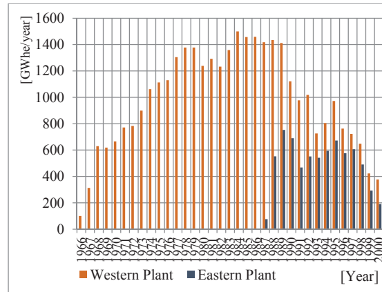
Fig. 6. Electricity generated by the cogeneration power plants of Oradea in the years 1966-2000 (GWh e /year).
