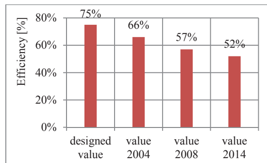
Fig. 17. Decreasing of the fuels overall efficiency usage at the Western Cogeneration Power Plant of Oradea in 2014 compared to the projected value.
