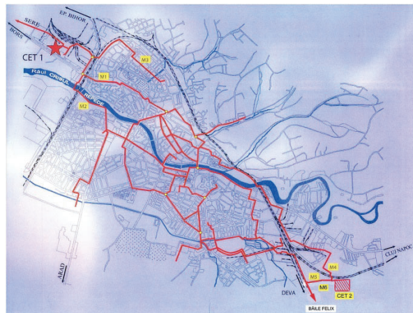
Fig. 11. District heating primary network operating at present in the city of Oradea.
