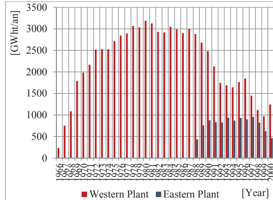
Fig. 8. Thermal energy production provided by the cogeneration power plants of Oradea, between 1966-2000.
