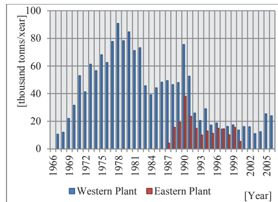
Fig. 4. Fuel-oil consumption registered by the cogeneration thermal plants of Oradea over the years 1967-2006.
