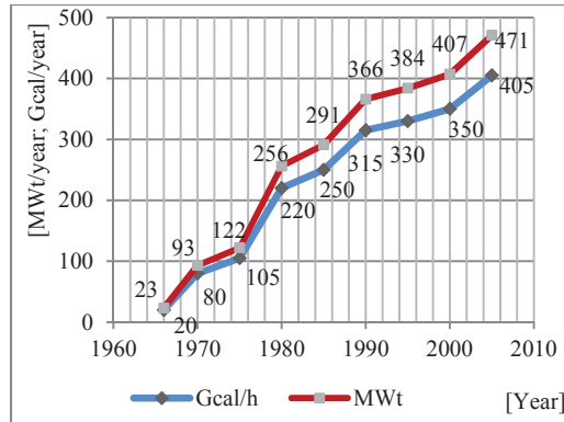
Fig. 14. Increasing the thermal power distribution capacities belonging to the district heating system of Oradea between 1966-2005.
