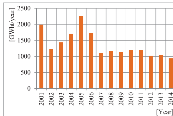
Fig. 9. Thermal energy delivered by the Western Cogeneration Plant of Oradea in form of technological steam and hot water over the years 2001-2014.
