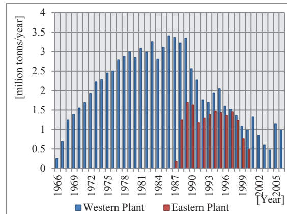
Fig. 3. Consumed coal at the cogeneration power plants of Oradea between 1966-2006.
